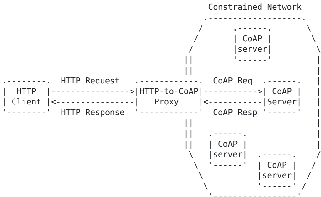
Figure 1: HTTP-To-CoAP Proxy Deployment Scenario
