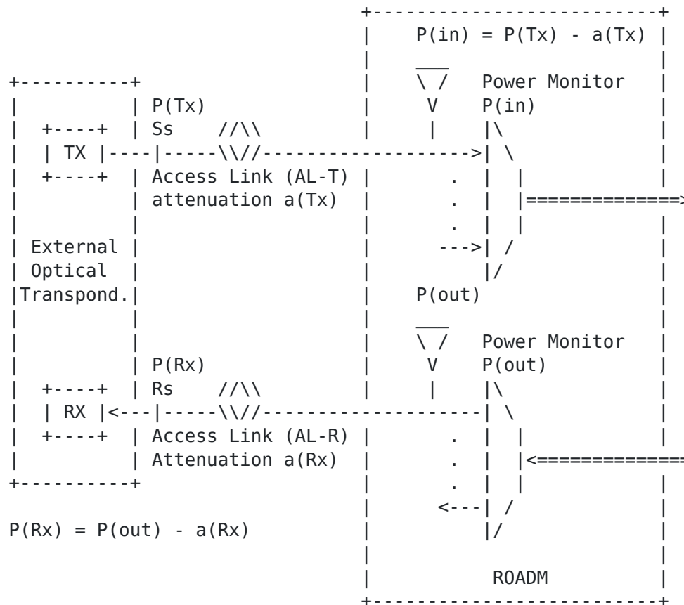
Figure 5 Access Link Power Monitoring
