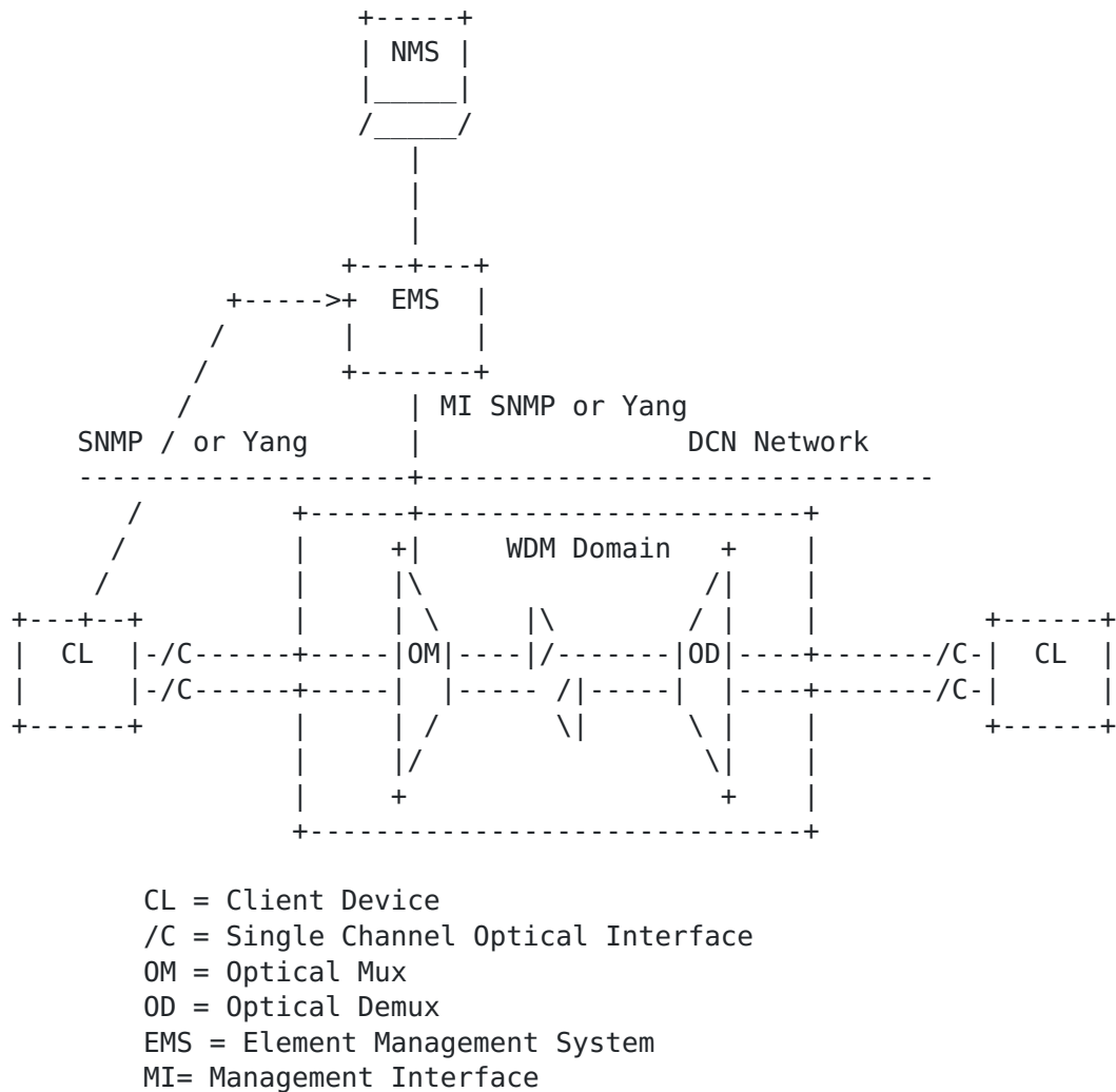
Figure 3: Connecting Single Channel optical interfaces to the Transport Management system
