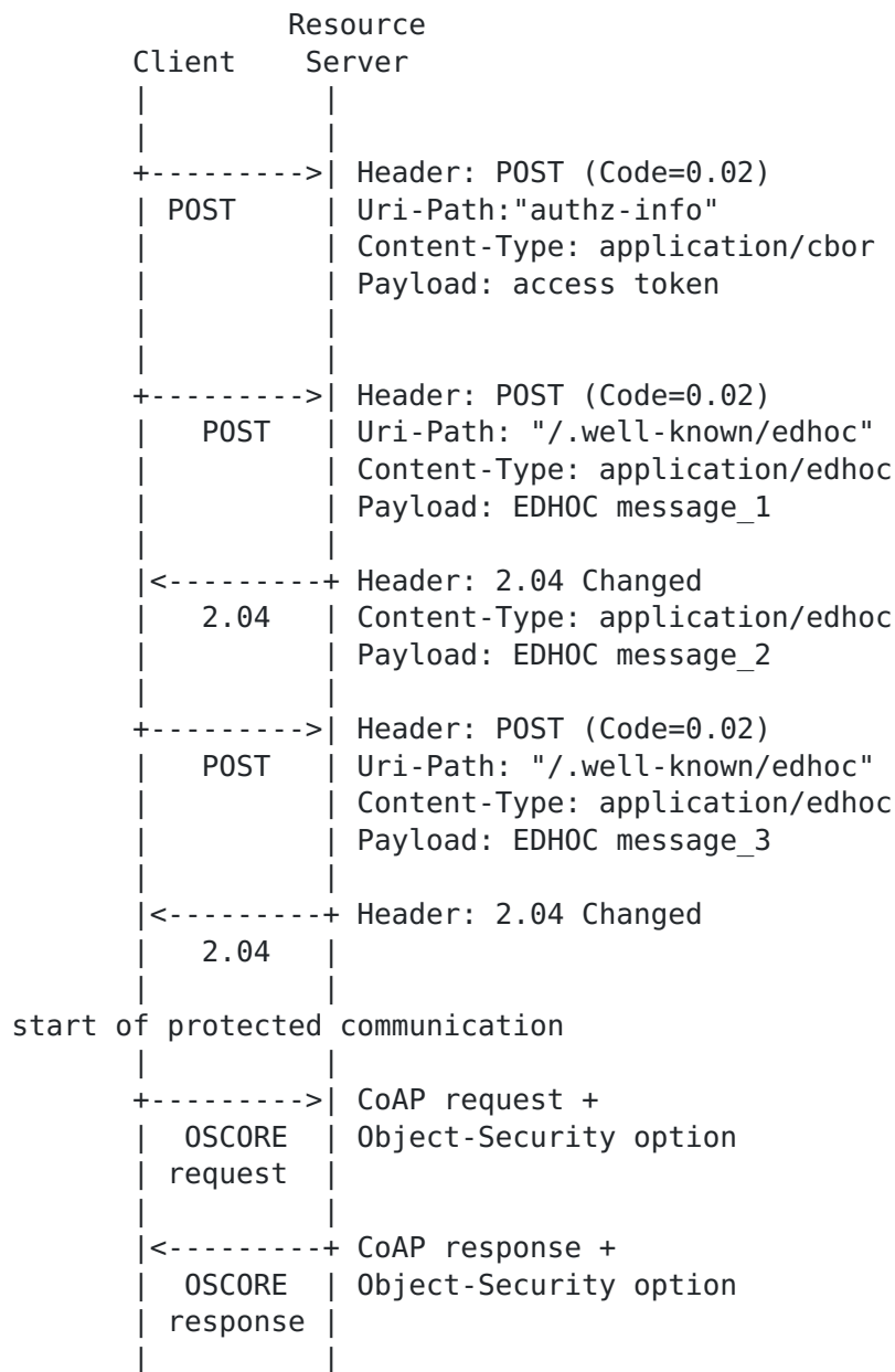
Figure 7: Access token and key establishment with EDHOC
