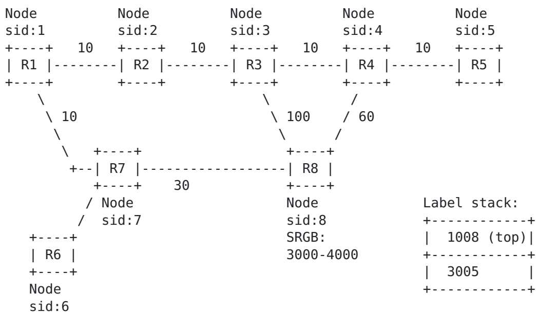
Figure 1: Example topology. The segment index for each node is shown in the diagram. All nodes have SRGB = [1000-2000], except for R8 which has SRGB = [3000-4000]. A label stack that represents the path R1->R7->R8->R4->R5 is shown as well.
