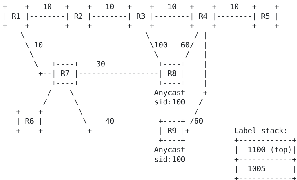
Figure 2: Topology illustrating use of anycast-sids to protect against node failures. All nodes have SRGB = [1000-2000].
