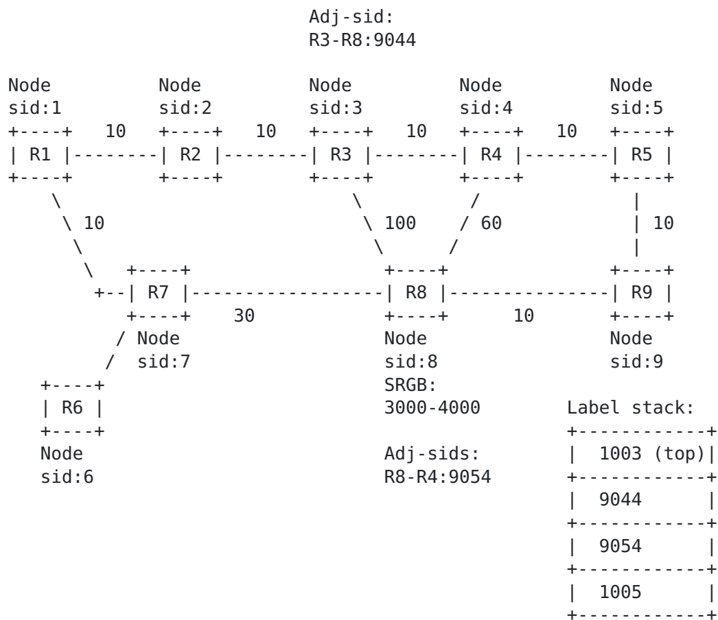
Figure 3: Explicit path using an adjacency sid. All nodes have SRGB = [1000-2000], except for R8 which has SRGB = [3000-4000].
