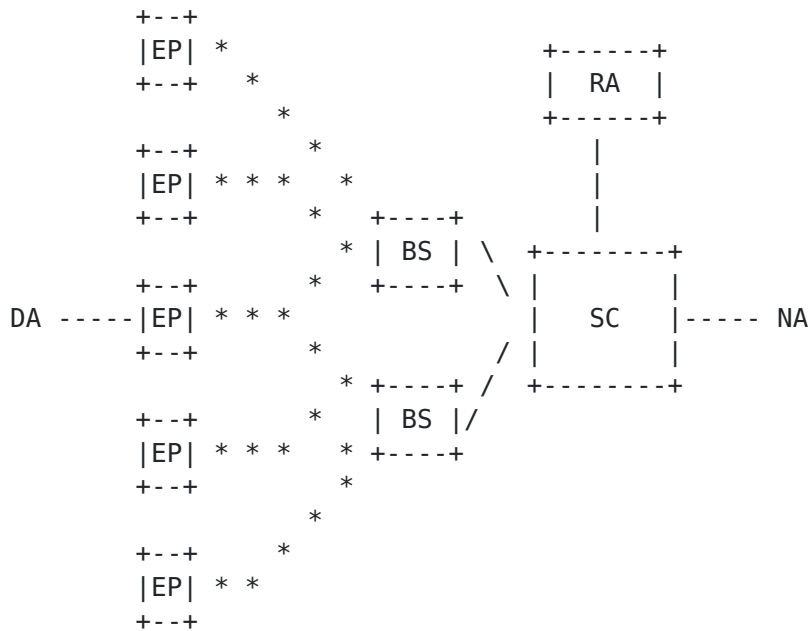
Figure 7: ETSI LTN architecture
