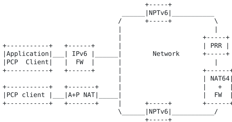
Figure 5: Multiple PCP-controlled devices
