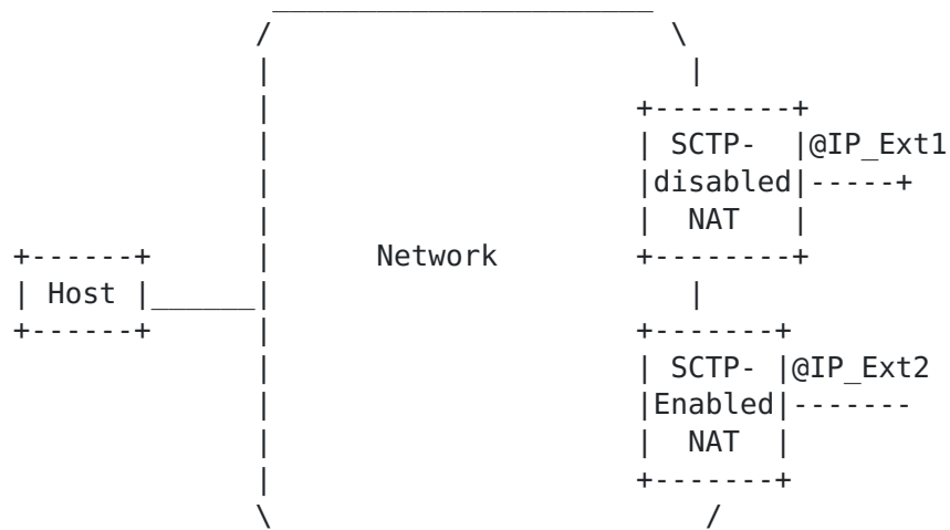
Figure 3: SCTP Example
